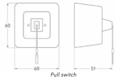
Pull switch
