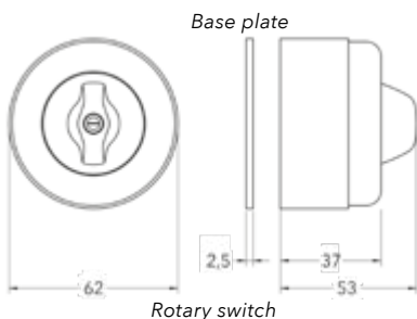
Rotary switch
